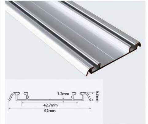
WSP-10 Sliding Bottom Profile
